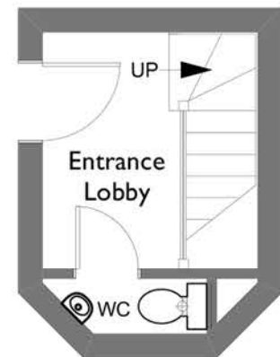
Ground Floor 6.68 sq. M
